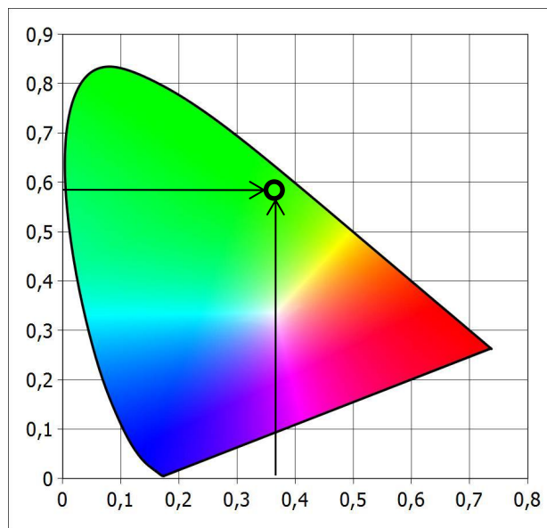
Diagram CIE 1931
